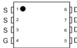
Pin Assignment
